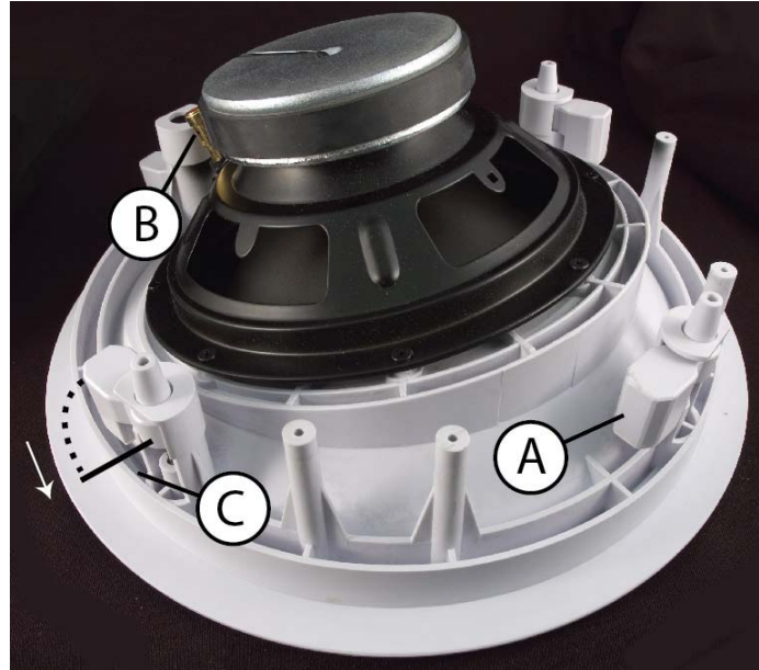
Rear View of Speaker Assembly
