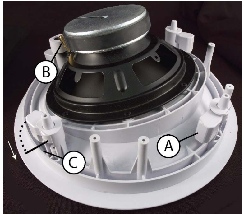
Rear View of Speaker Assembly
