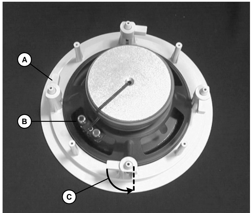
Rear View of Speaker Assembly
